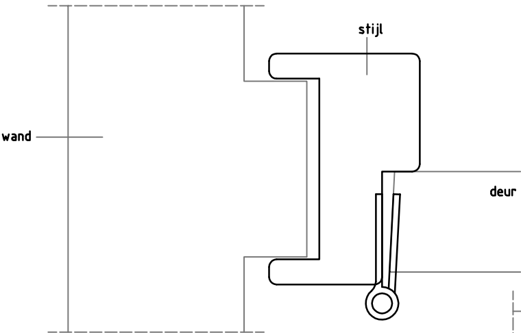
Detail 1: stijl
