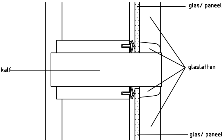
Detail 6: kalf
