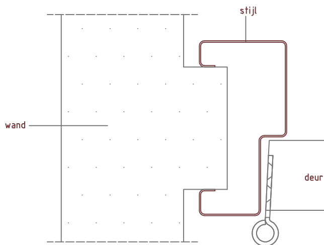
Detail 1: stijl
