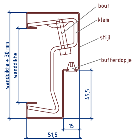
Detail 2: klem
