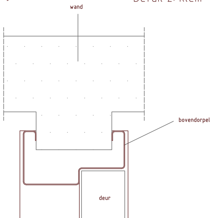
Detail 2: klem
