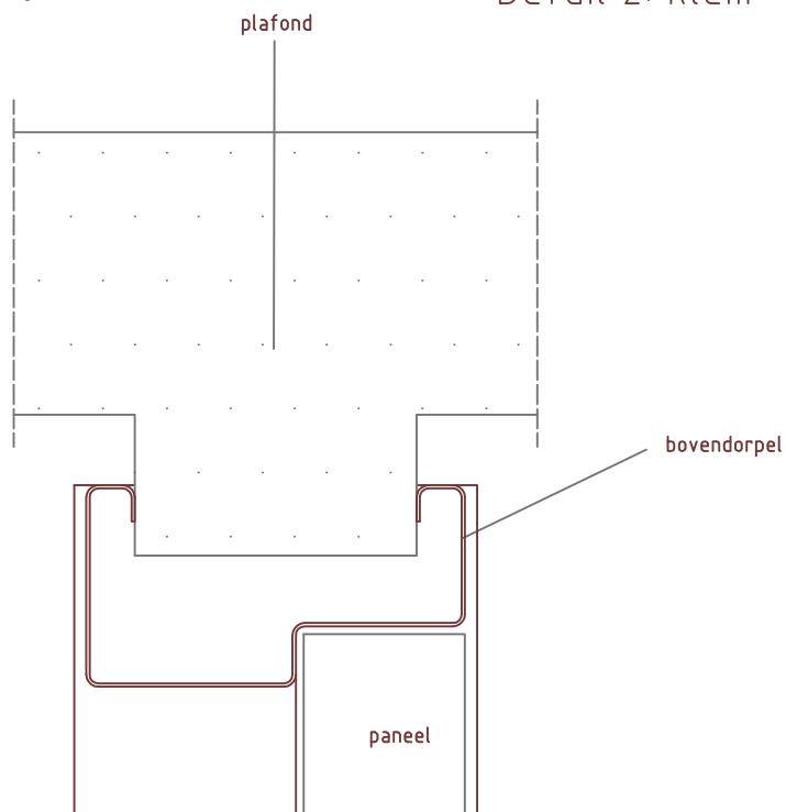
Detail 2: klem
