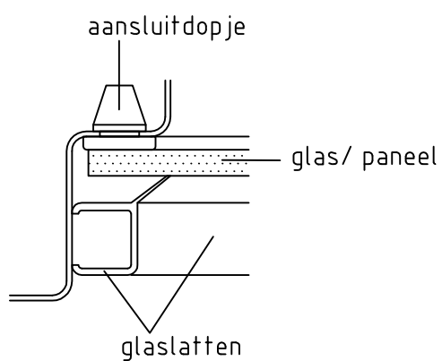
Detail 7: glaslat
