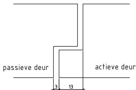
Detail 5: sponning-contrasponning
