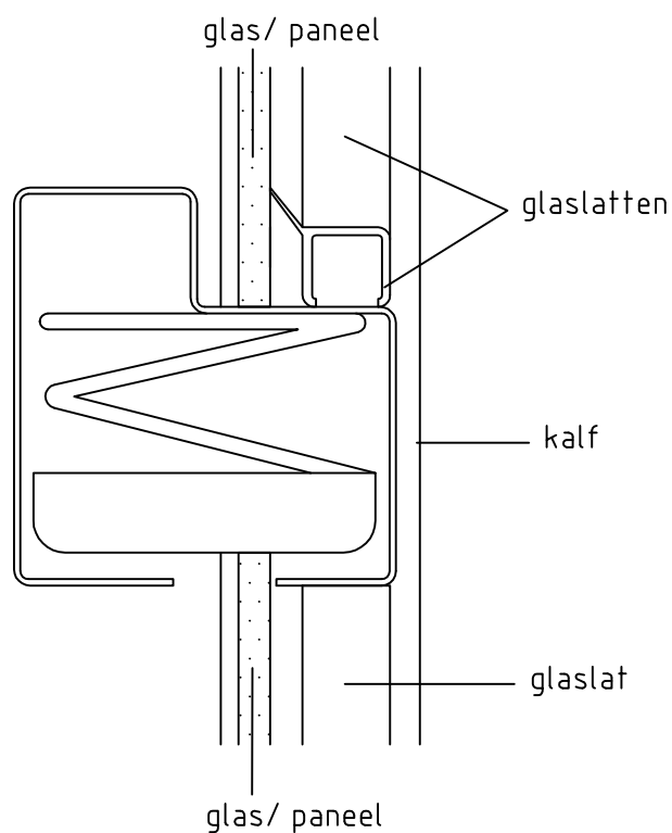
Detail 8: kalf
