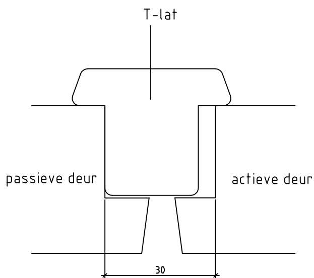
Detail 4: T-lat
