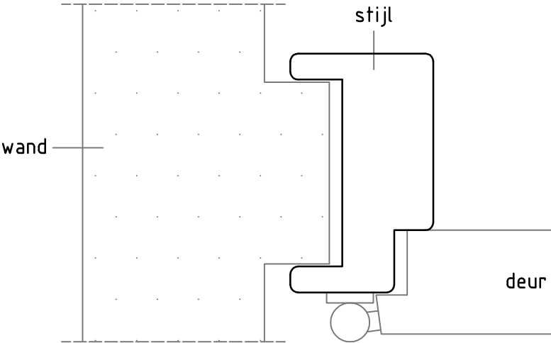
Detail 1: stijl
