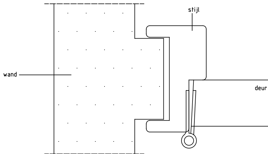
Detail 1: stijl
