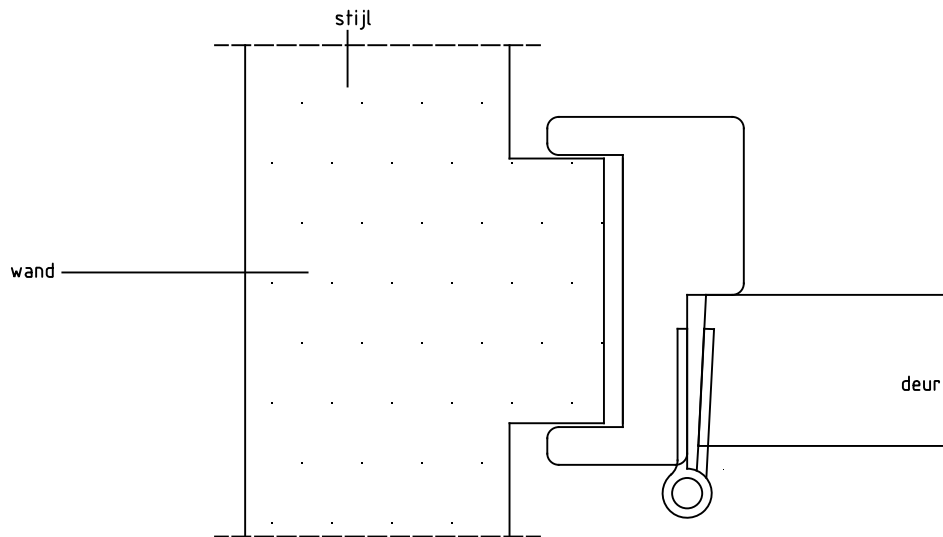
Detail 1: stijl
