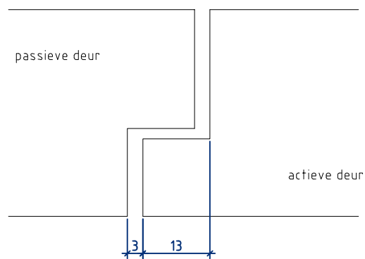
Detail 5: sponning-contrasponning
