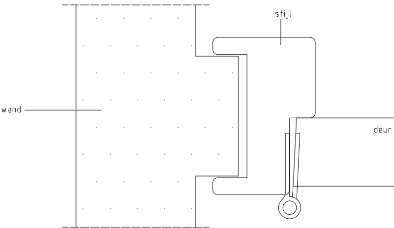
Detail 1: stijl
