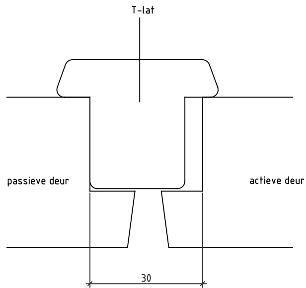
Detail 3: T-lat
