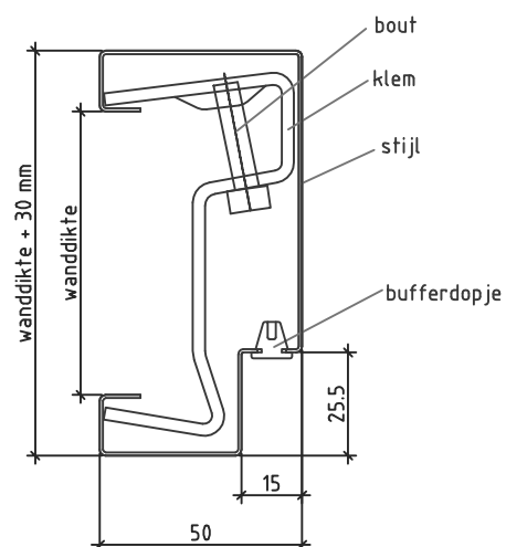
Detail 2: klem
