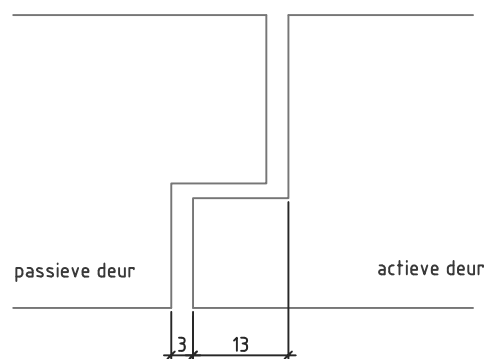
Detail 5: sponning-contrasponning
