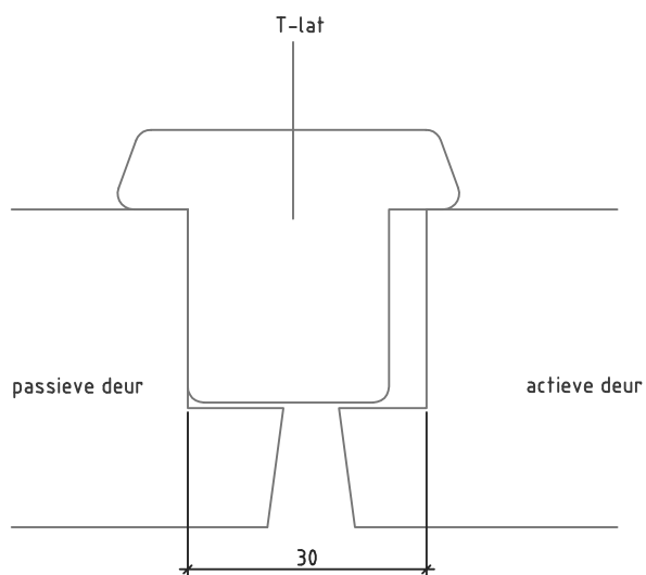
Detail 4: T-lat
