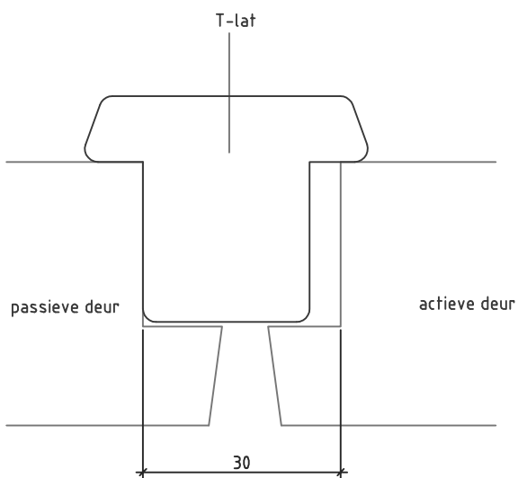
Detail 4: T-lat
