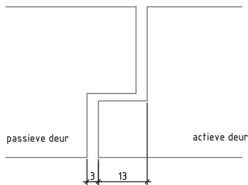
Detail 5: sponning-contrasponning
