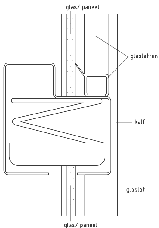
Detail 8: kalf
