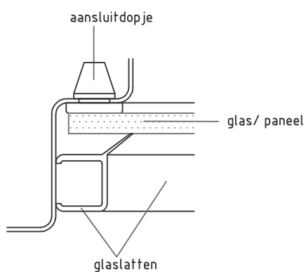
Detail 7: glaslat
