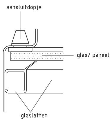
Detail 6: glaslat
