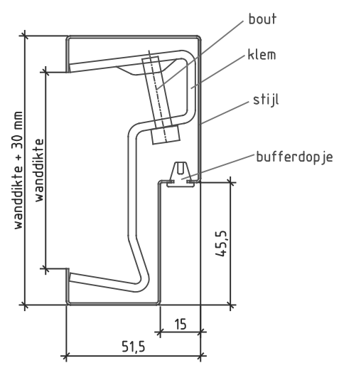
Detail 2: klem
