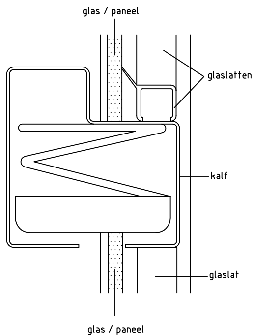
Detail 8: kalf
