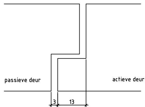
Detail 6: sponning-contrasponning
