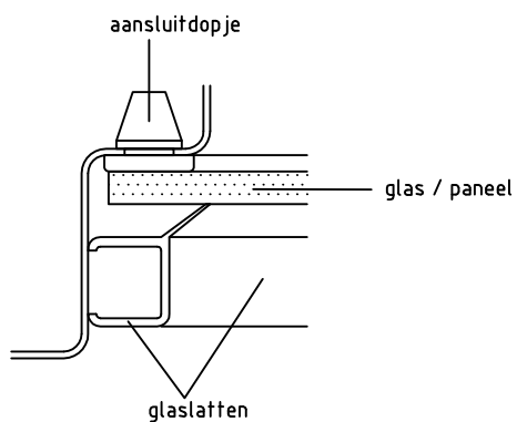
Detail 7: glaslat
