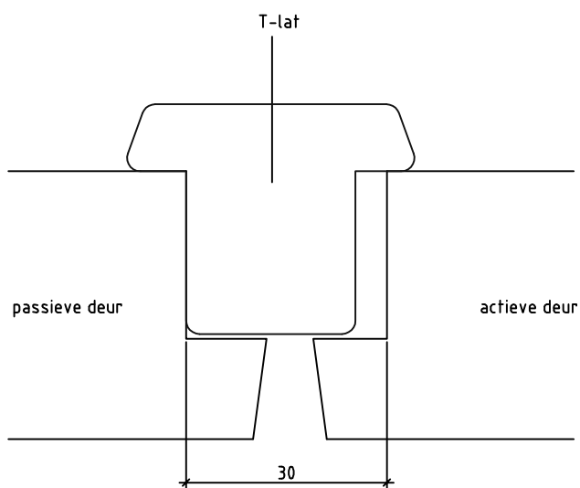
Detail 5: T-lat
