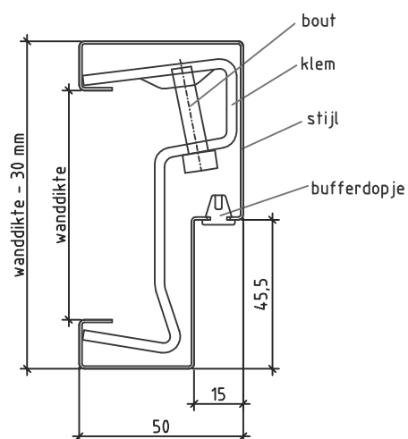
Detail 2: klem
