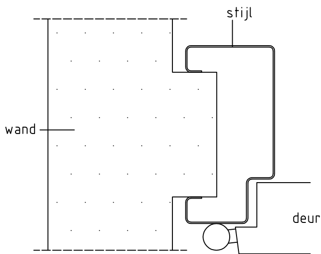
Detail 1: stijl
