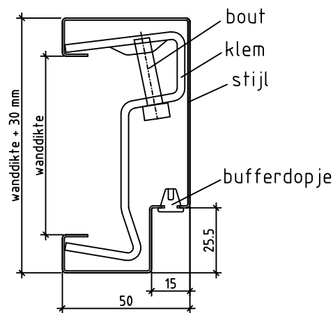
Detail 2: klem
