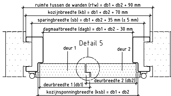
Doorsnede AA spooning/contraspooning
