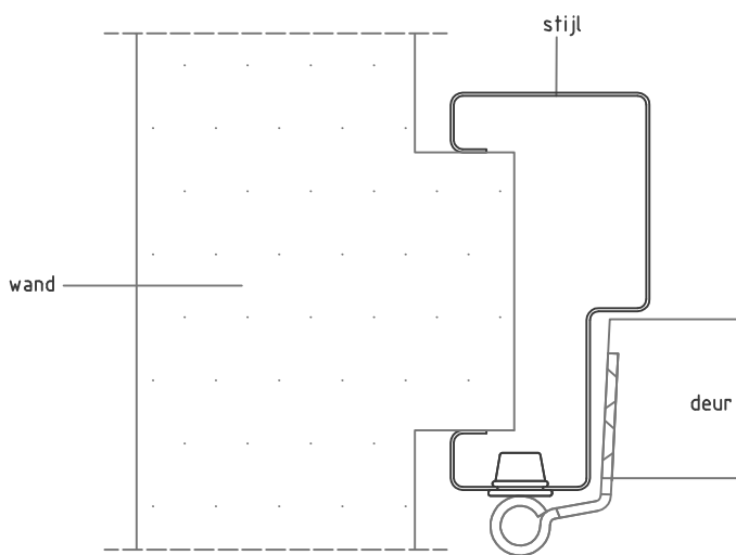
Detail 1: stijl
