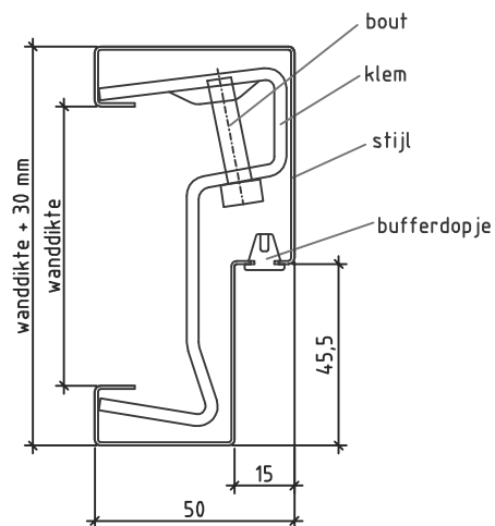
Detail 2: klem
