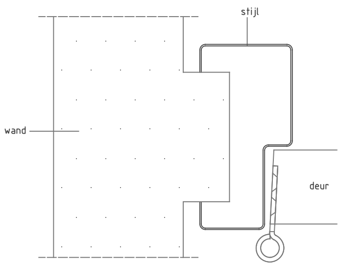
Detail 1: stijl
