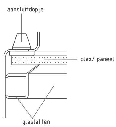
Detail 6: glaslat
