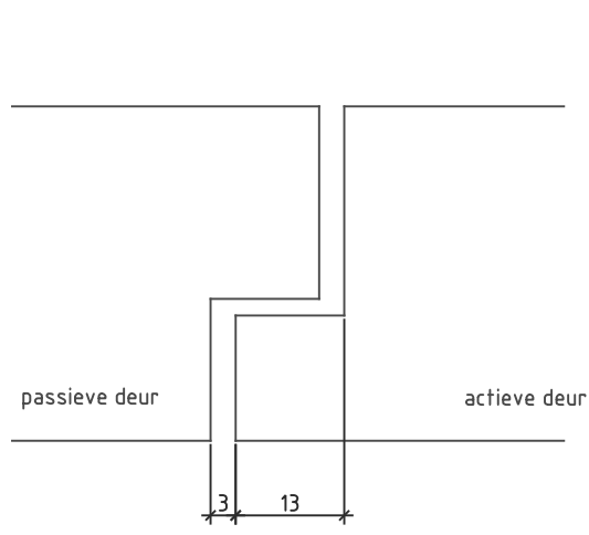
Detail 4: sponning-contrasponning
