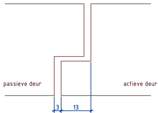
Detail 4: sponning-contrasponning
