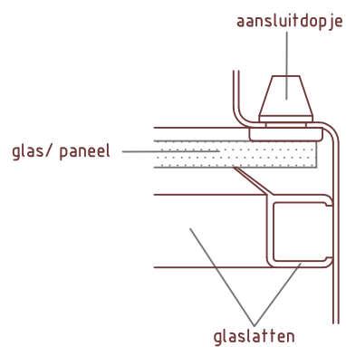
Detail 5: glaslat
